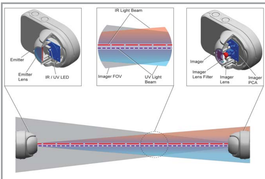
OSID Operational Diagram
