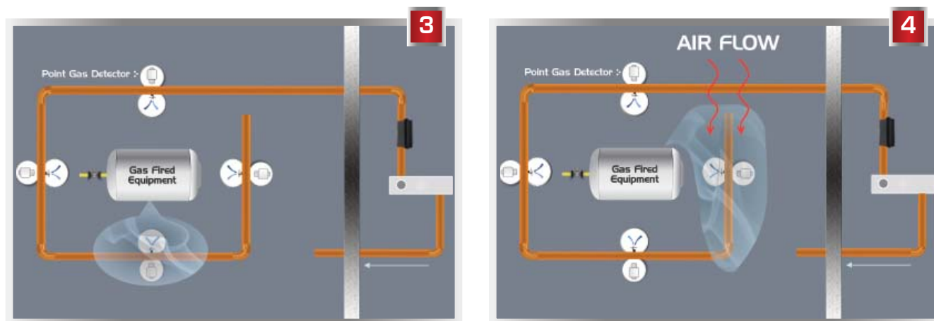
Figures 3 + 4 — Demonstrate the design flexibility of VESDA ECO. Knowing where a leak will occur is always a judgement call. In this example, four conventional point gas detectors are required to cover the same area as one VESDA ECO detector. VESDA ECO provides a more cost-effective solution.
